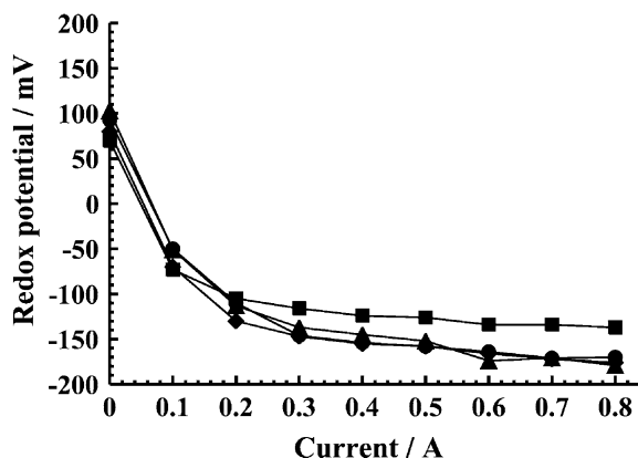
Fig. 5. The relationship between redox potential (mV) and electric current (A) using various electrolyte solutions. (●) NaCl, (▲) KCl, (◆) \text{MgCl}_2 and (■) \text{CaCl}_2 .
