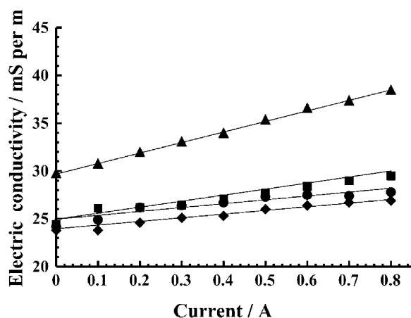
Fig. 3. The relationship between electric conductivity (mS per m) and electric current (A) using various electrolyte solutions. (●) NaCl, (▲) KCl, (◆) \text{MgCl}_2 and (■) \text{CaCl}_2 .
