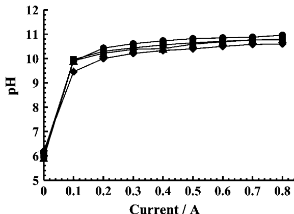
Fig. 4. The relationship between pH and electric current (A) using various electrolyte solutions. (●) NaCl, (▲) KCl, (◆) \text{MgCl}_2 and (■) \text{CaCl}_2 .
